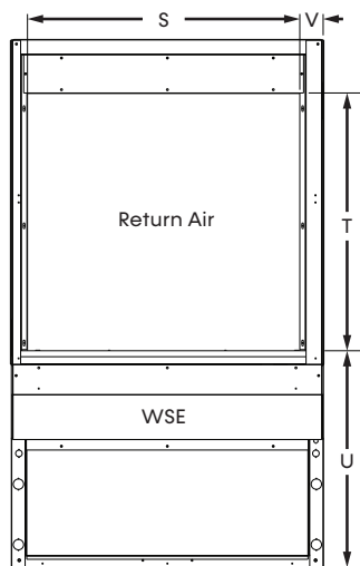
Back View Rear Return Front Discharge
